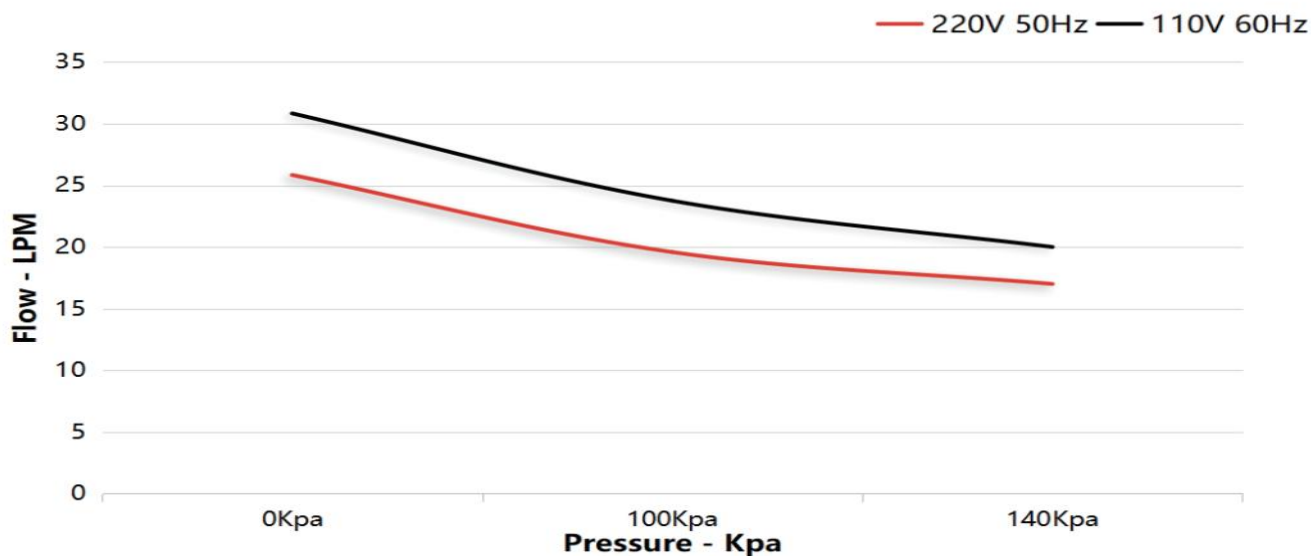
Performance Chart - Flow VS. Pressure
