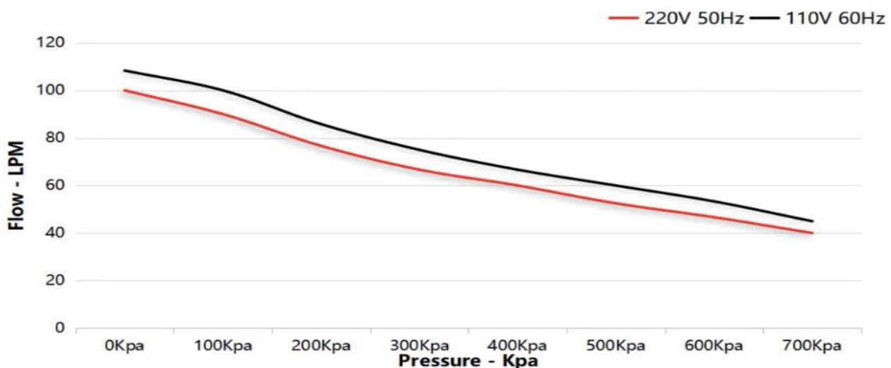
Performance Chart - Flow VS. Pressure
